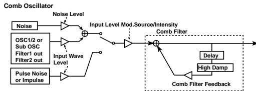
Example of when noise is input
