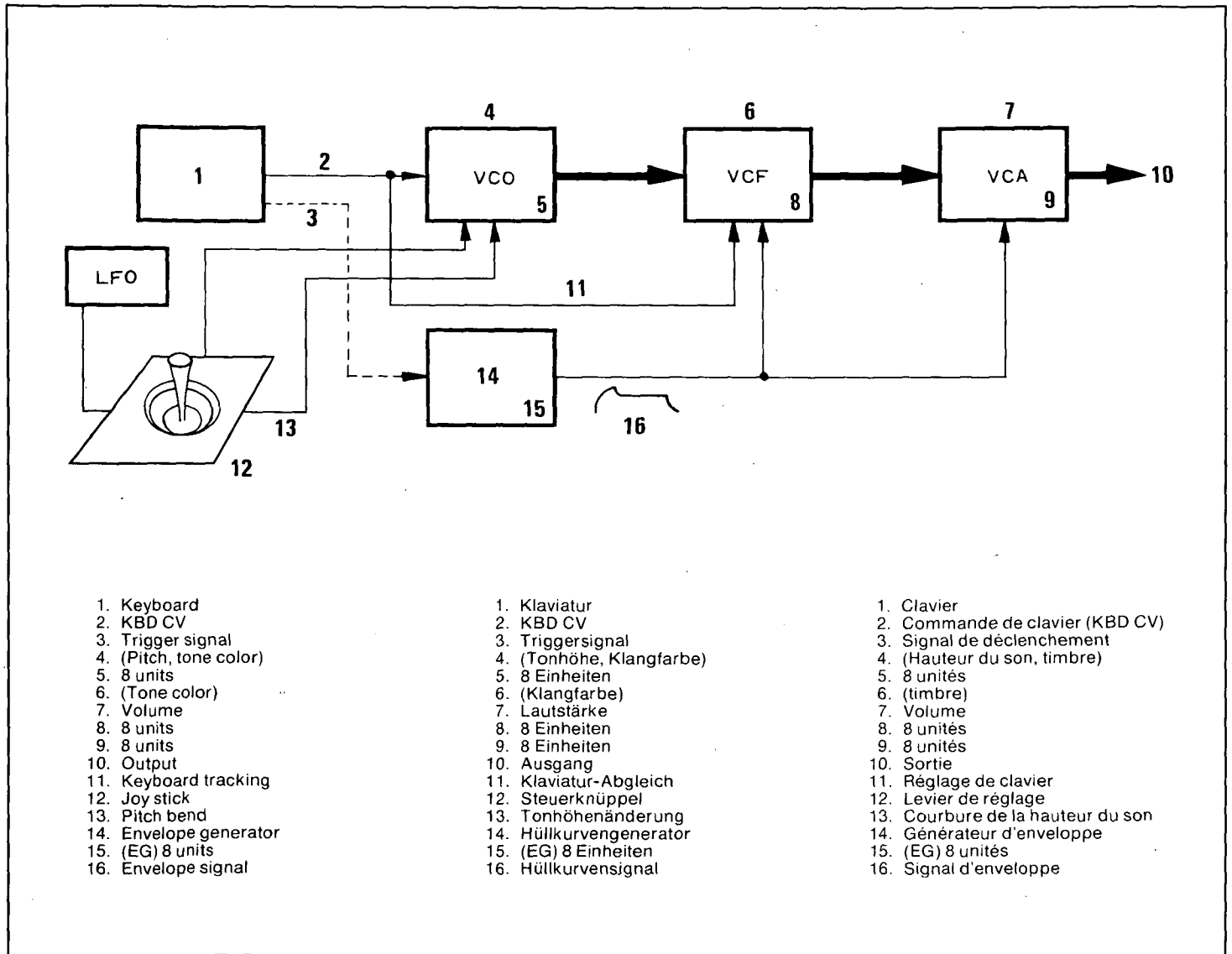
Block diagram of synthesizer
