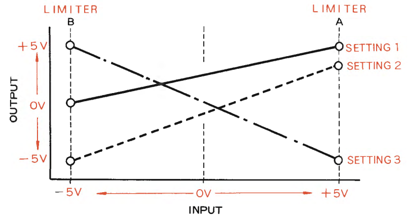
fig.32(B) VP operation(VPの動作)
