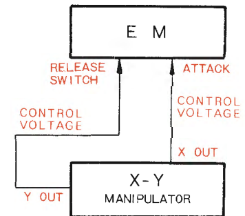
fig. 54 Block diagram of manual envelope control.
