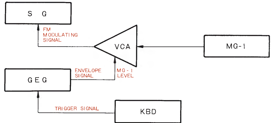
fig. 50 Delayed vibrato block diagram.
