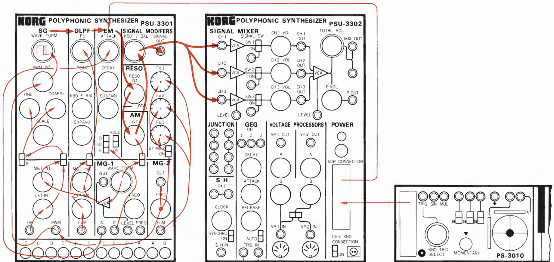
fig.40 signal flow (信号の流れ)
