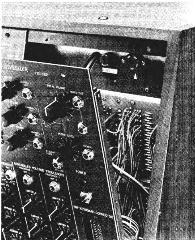
Fig. 57 Power supply voltage selector and fuse holder. (電源電圧セレクターとFUSEホルダー)
