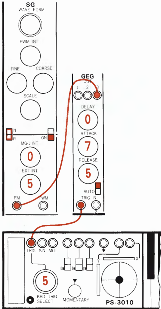
fig.28 Five key bend (5thベンド)
