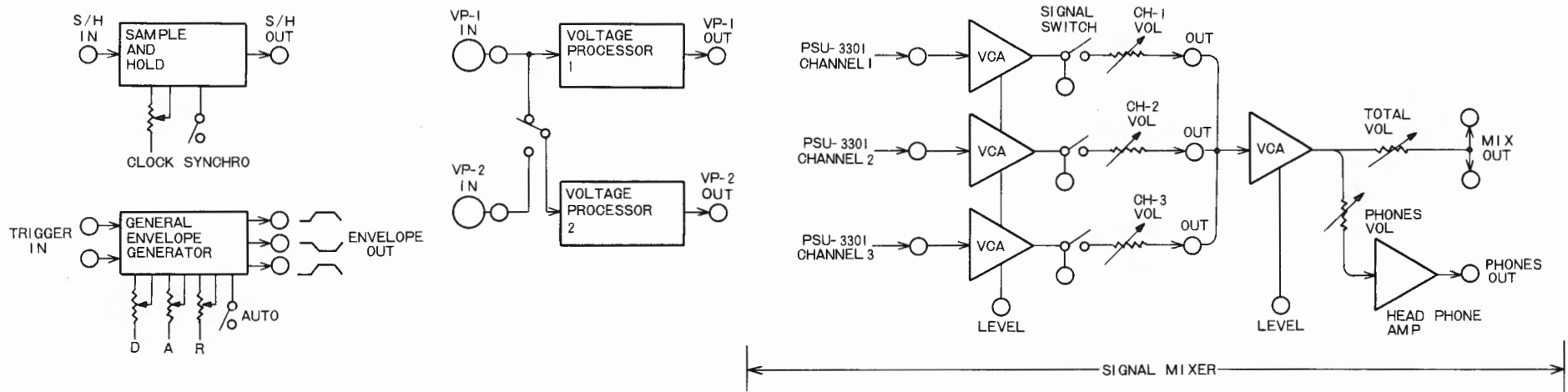
fig.2(B) PSU-3302(MIXER)
