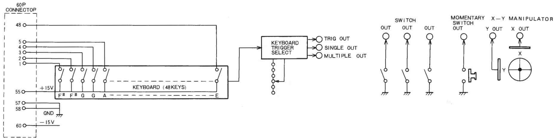
fig.2(C) PS-3010(KEYBOARD)
