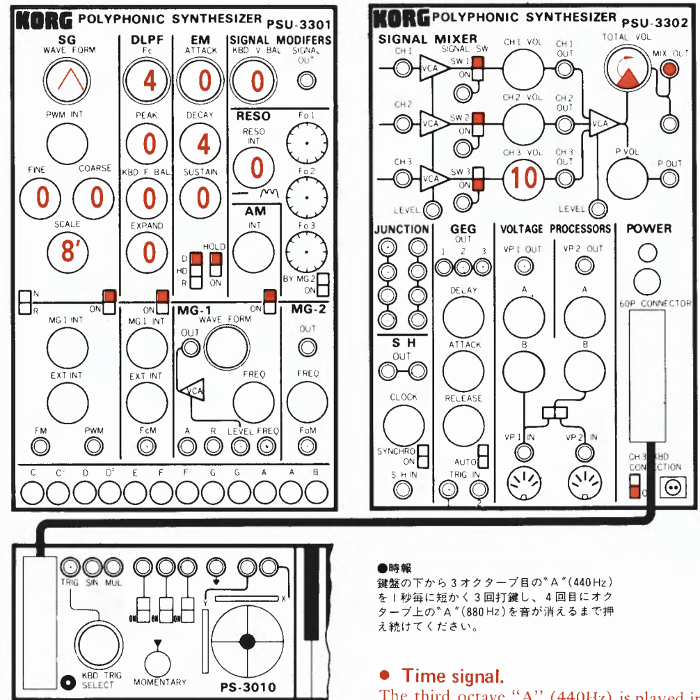
fig.39 Time signal (時報の実験)
