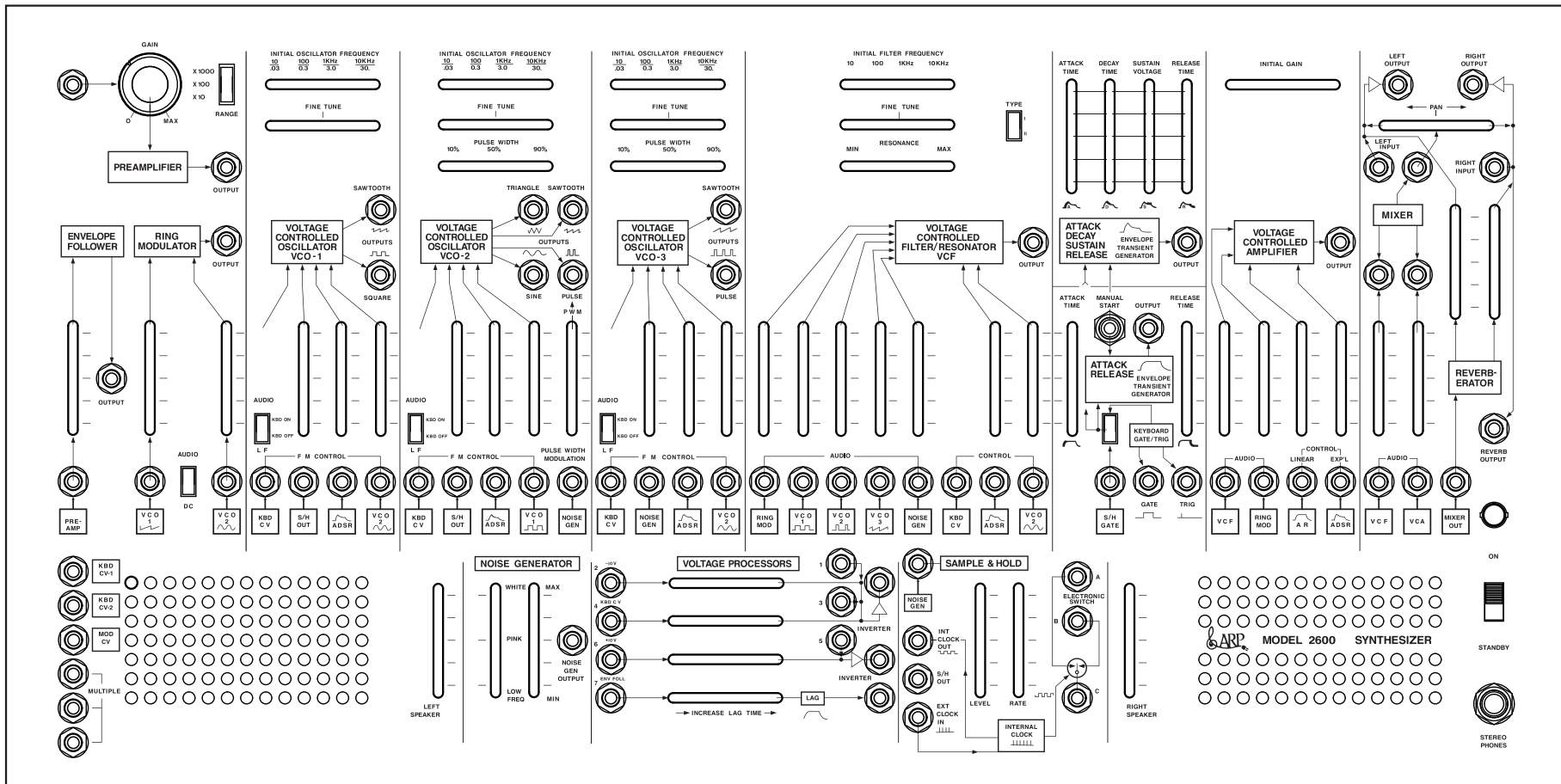
2600 M FRONT PANEL FACSIMILE
