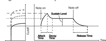
Figure 9-1: EG Intensity
