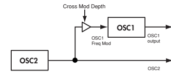
Figure 5-1: Cross Mod
