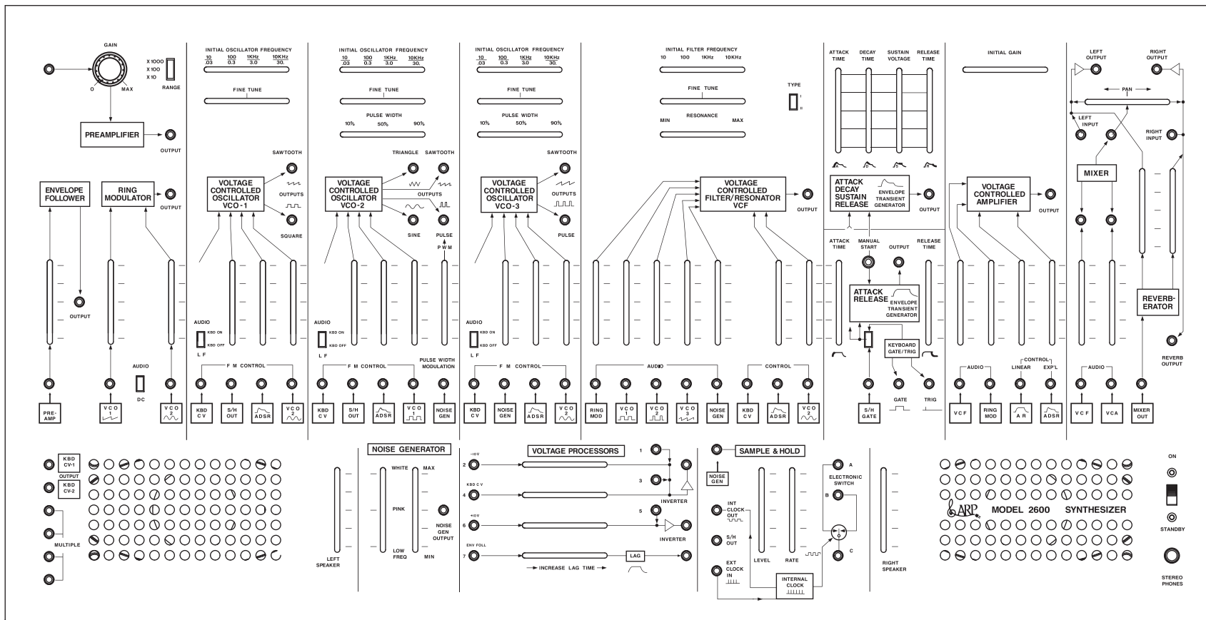
2600 FS FRONT PANEL FACSIMILE
