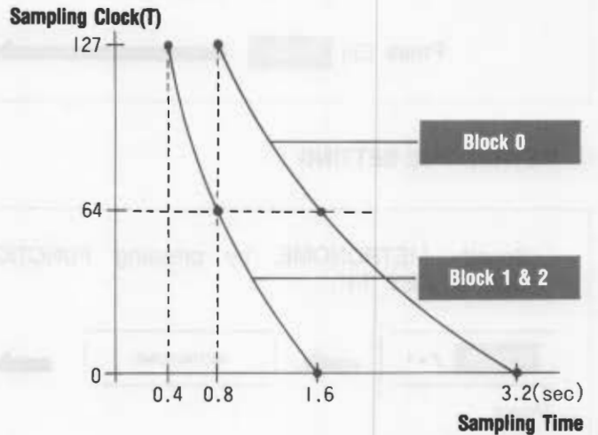
Relationship between Sampling Clock and Sampling Time
